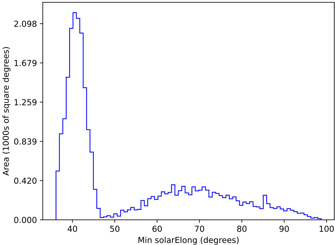
mw_roll_all_v3.3_10yrs All sky i band: Min solarElong
