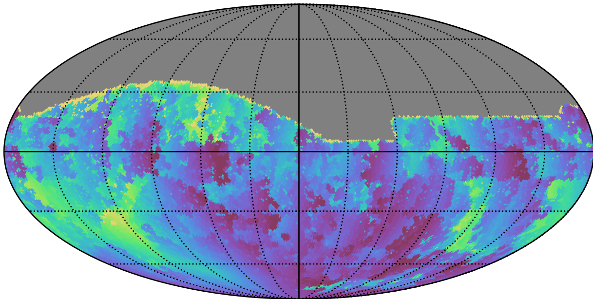
mw_roll_all_v3.3_10yrs All sky g band: Min solarElong
