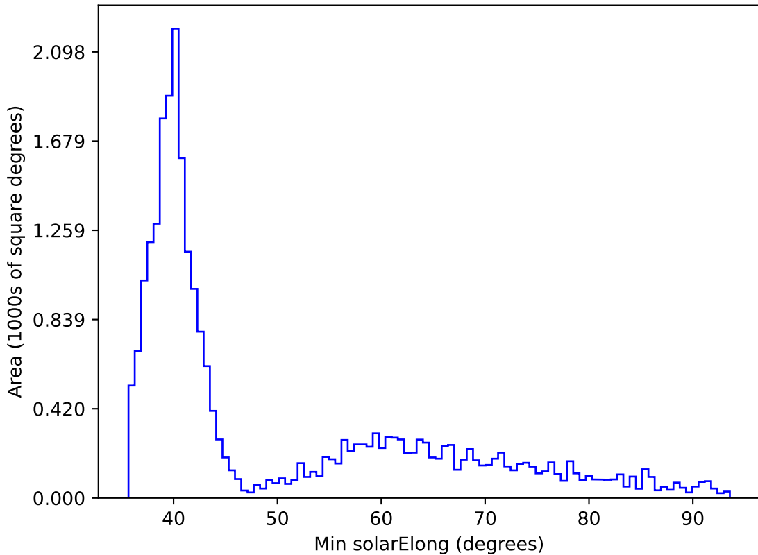
mw_roll_all_v3.3_10yrs All sky all bands: Min solarElong
