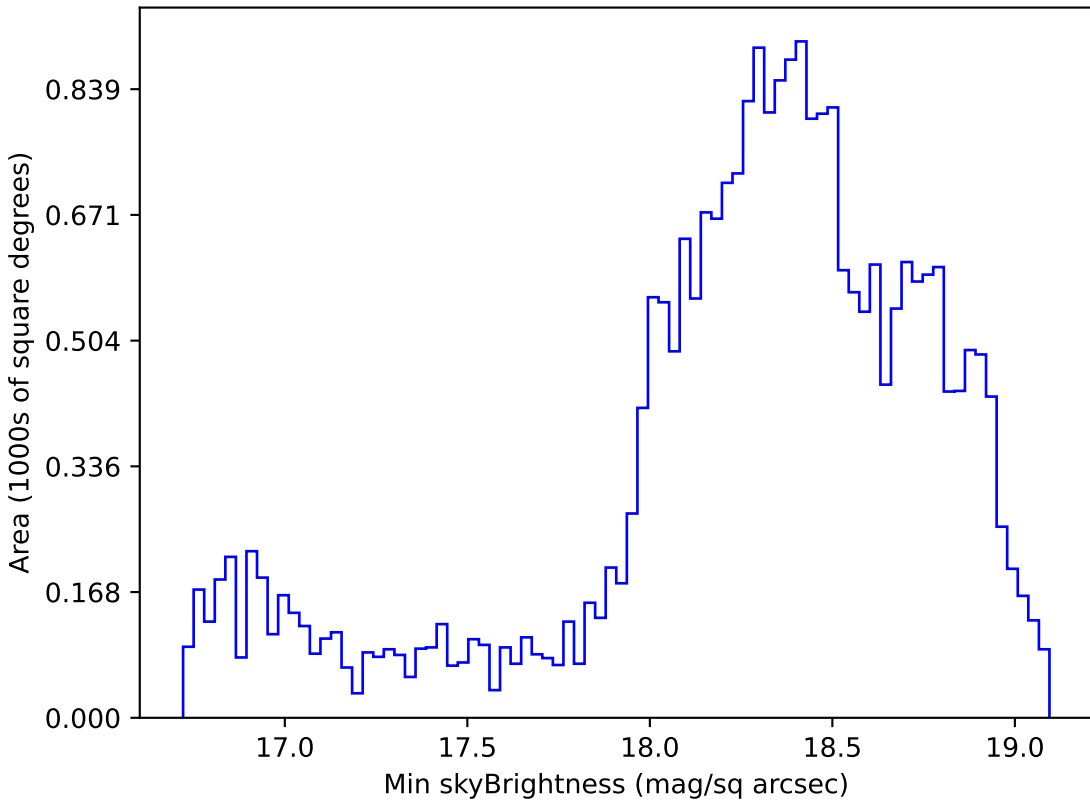
mw_roll_all_v3.3_10yrs Yr 1 z band: Min skyBrightness
