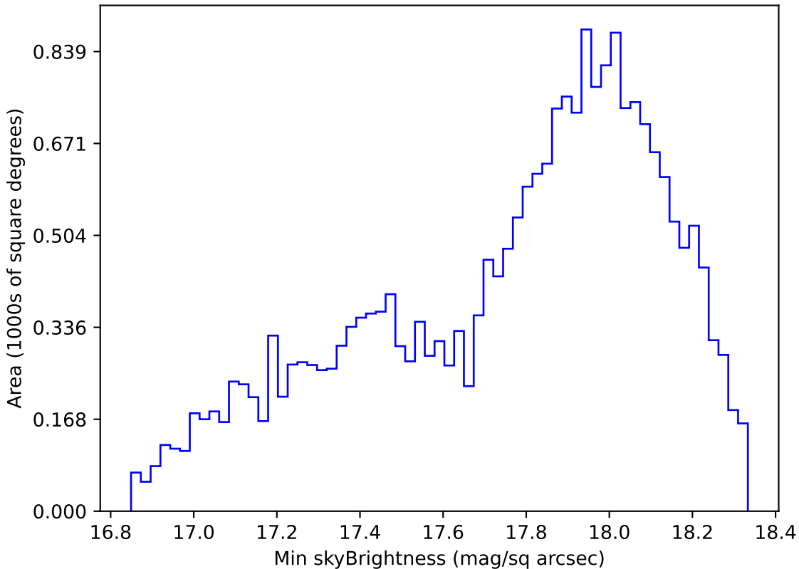
mw_roll_all_v3.3_10yrs Yr 1 y band: Min skyBrightness
