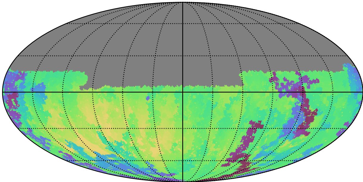
mw_roll_all_v3.3_10yrs Yr 1 u band: Min skyBrightness
