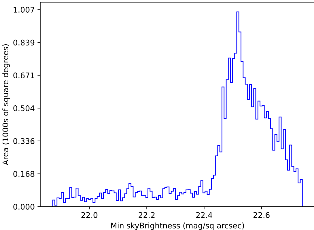
mw_roll_all_v3.3_10yrs Yr 1 u band: Min skyBrightness
