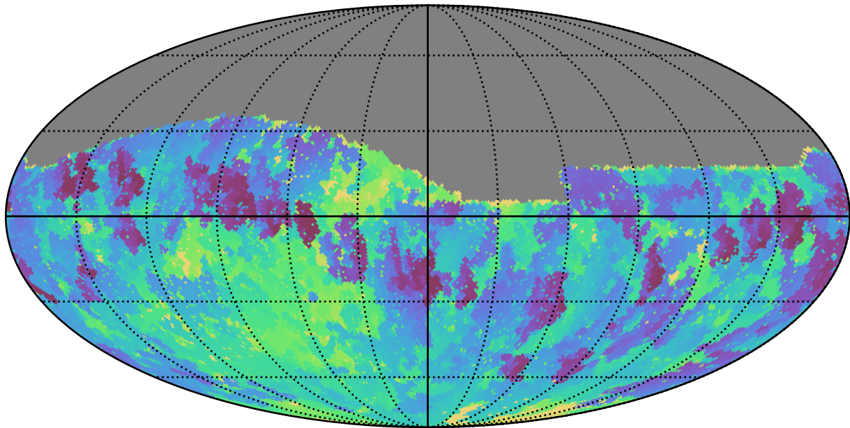
mw_roll_all_v3.3_10yrs Yr 1 i band: Min skyBrightness
