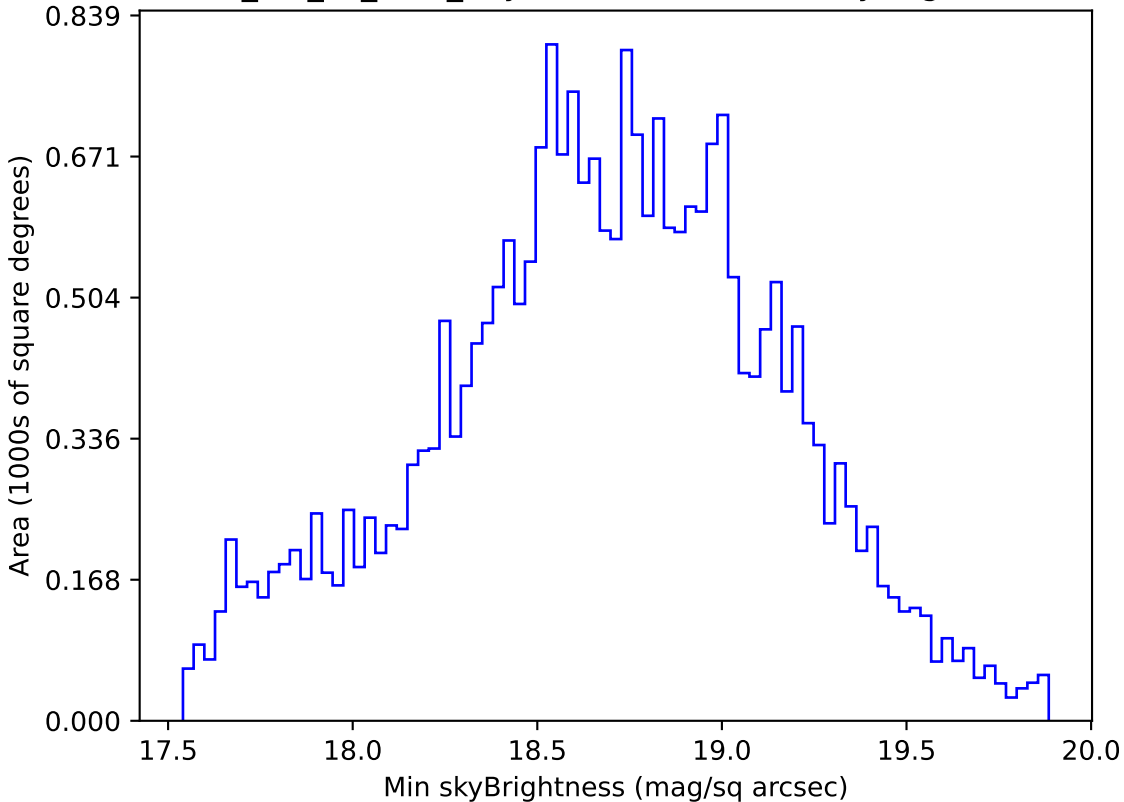
mw_roll_all_v3.3_10yrs Yr 1 i band: Min skyBrightness
