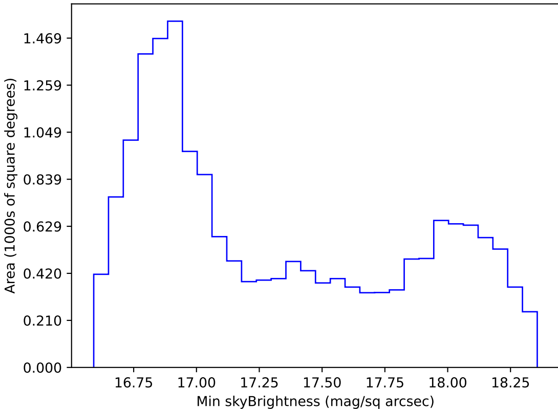
mw_roll_all_v3.3_10yrs WFD z band: Min skyBrightness
