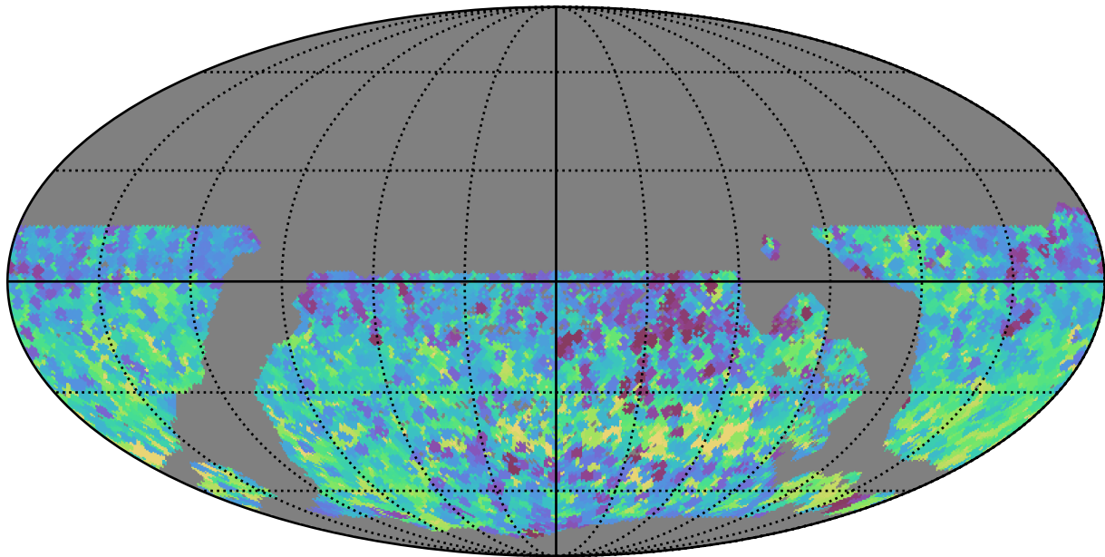
mw_roll_all_v3.3_10yrs WFD y band: Min skyBrightness
