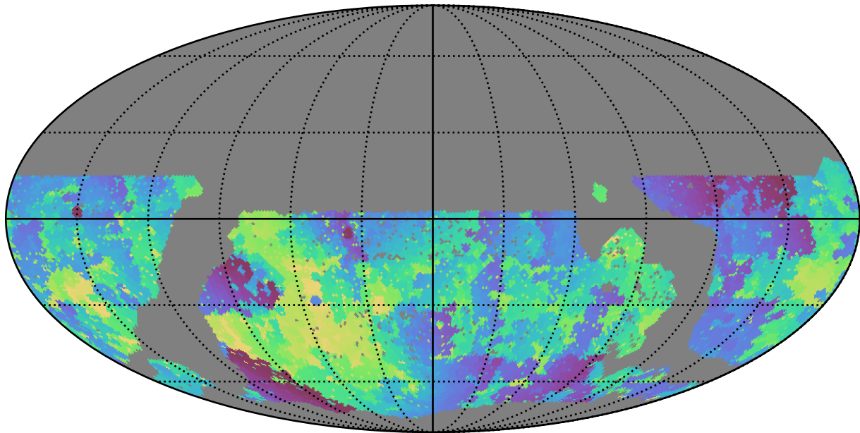
mw_roll_all_v3.3_10yrs WFD u band: Min skyBrightness
