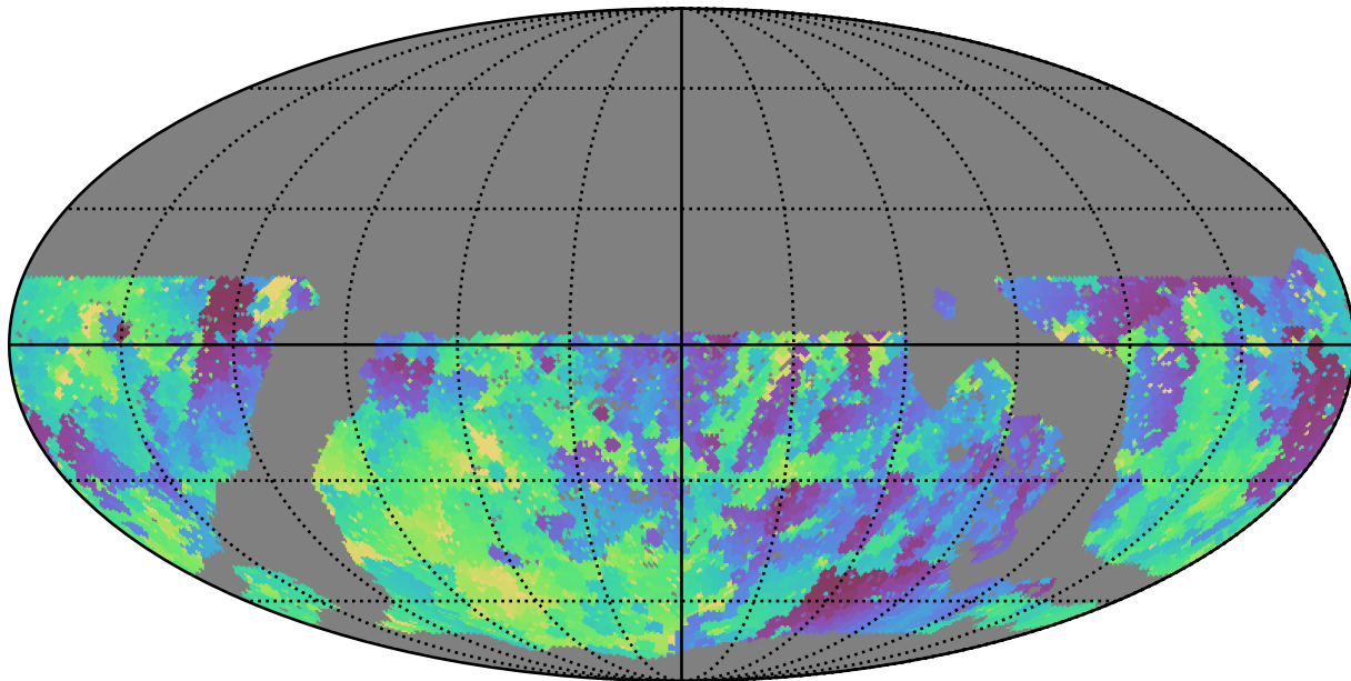
mw_roll_all_v3.3_10yrs WFD r band: Min skyBrightness
