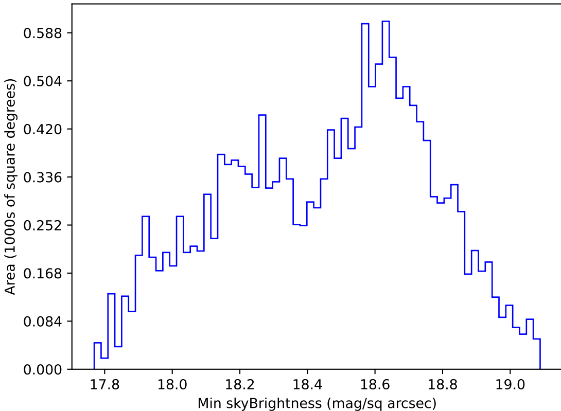
mw_roll_all_v3.3_10yrs WFD r band: Min skyBrightness
