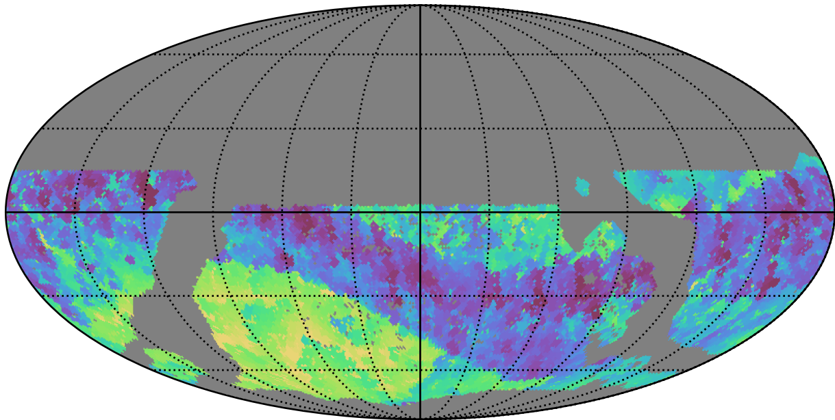
mw_roll_all_v3.3_10yrs WFD i band: Min skyBrightness
