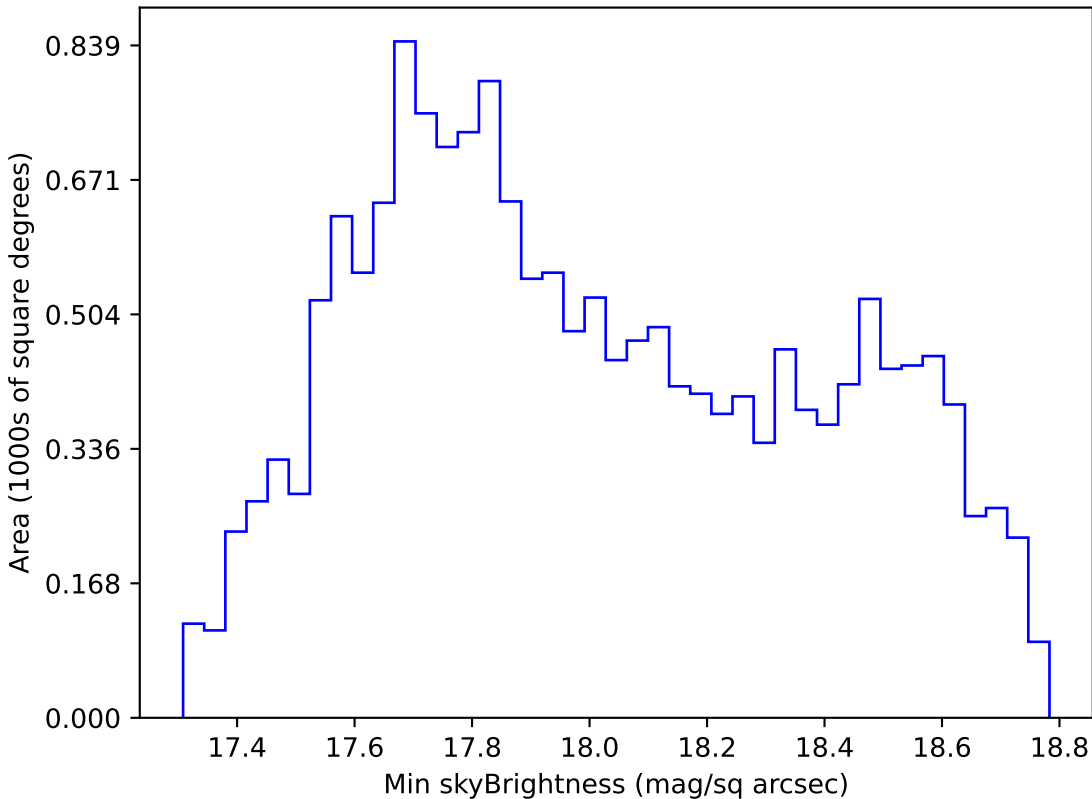
mw_roll_all_v3.3_10yrs WFD i band: Min skyBrightness
