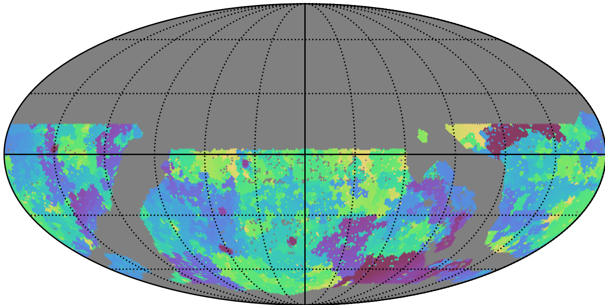
mw_roll_all_v3.3_10yrs WFD g band: Min skyBrightness
