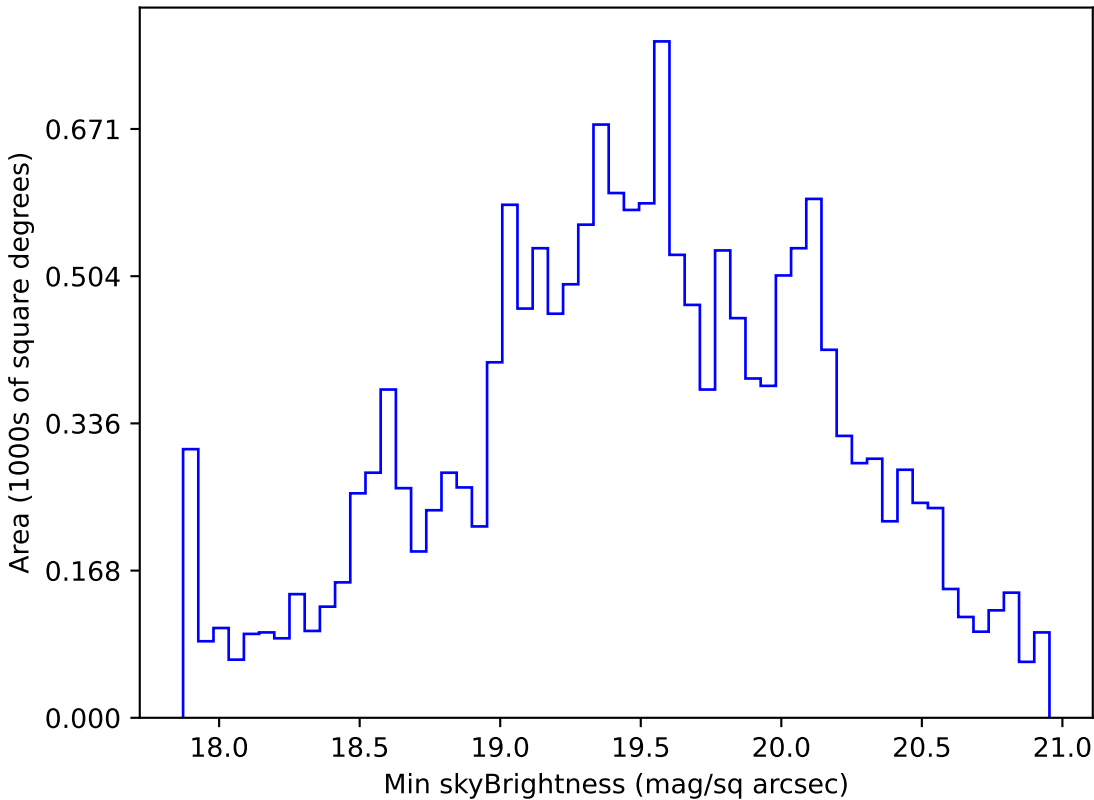
mw_roll_all_v3.3_10yrs WFD g band: Min skyBrightness
