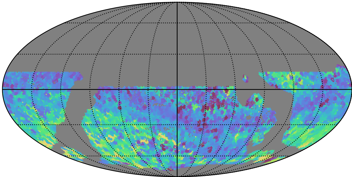
mw_roll_all_v3.3_10yrs WFD all bands: Min skyBrightness
