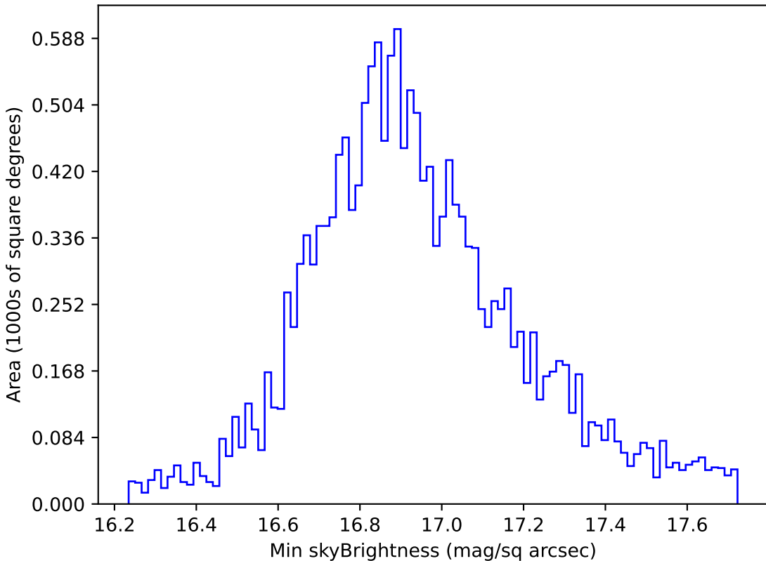
mw_roll_all_v3.3_10yrs WFD all bands: Min skyBrightness
