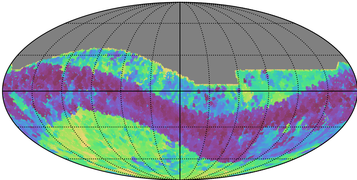
mw_roll_all_v3.3_10yrs All sky z band: Min skyBrightness
