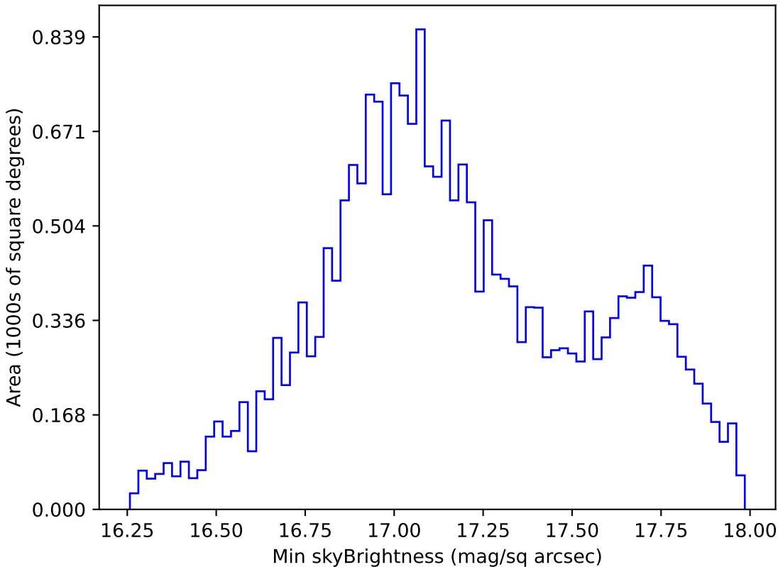
mw_roll_all_v3.3_10yrs All sky y band: Min skyBrightness
