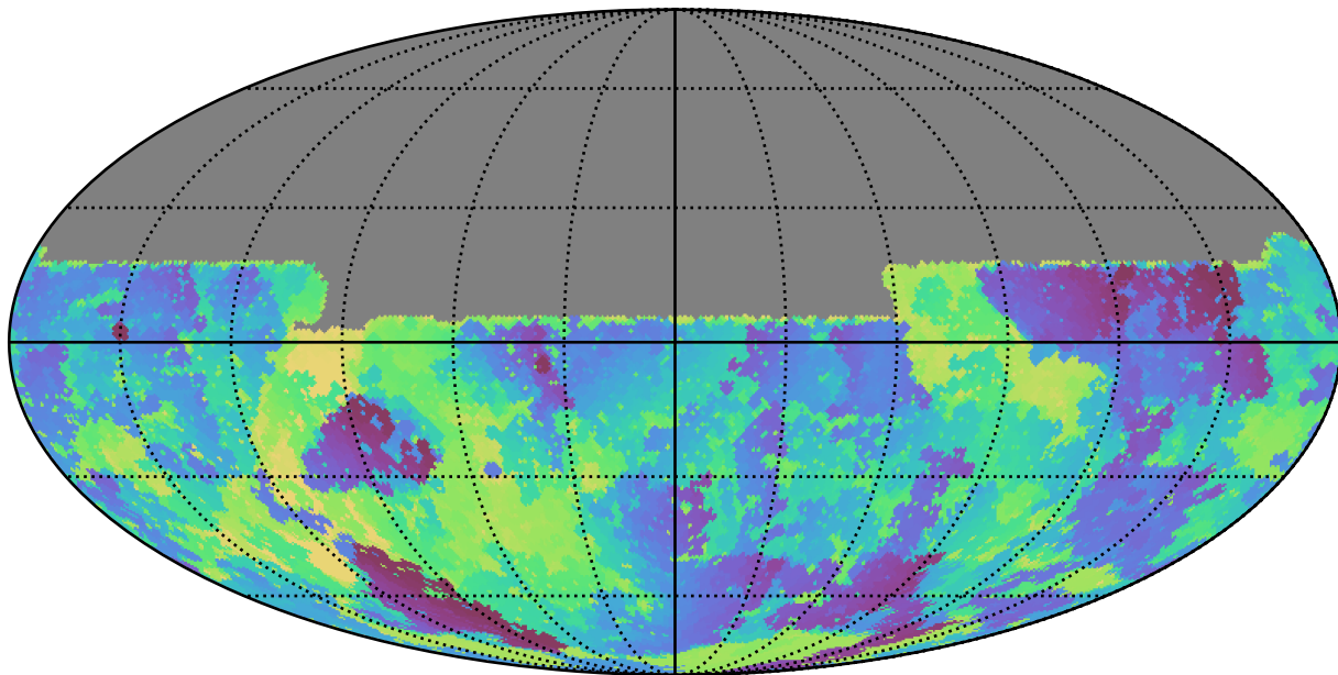
mw_roll_all_v3.3_10yrs All sky u band: Min skyBrightness
