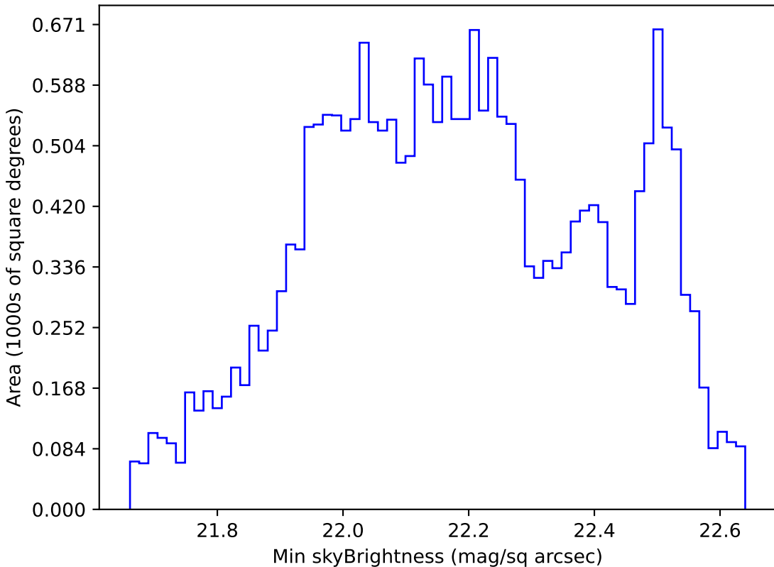
mw_roll_all_v3.3_10yrs All sky u band: Min skyBrightness
