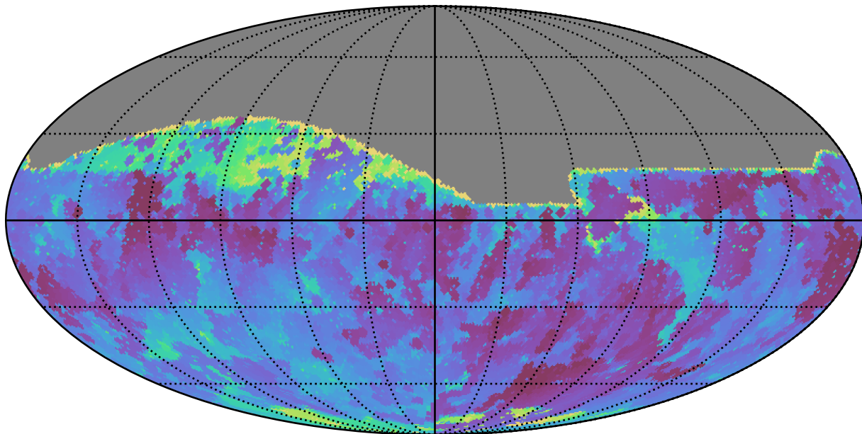
mw_roll_all_v3.3_10yrs All sky r band: Min skyBrightness
