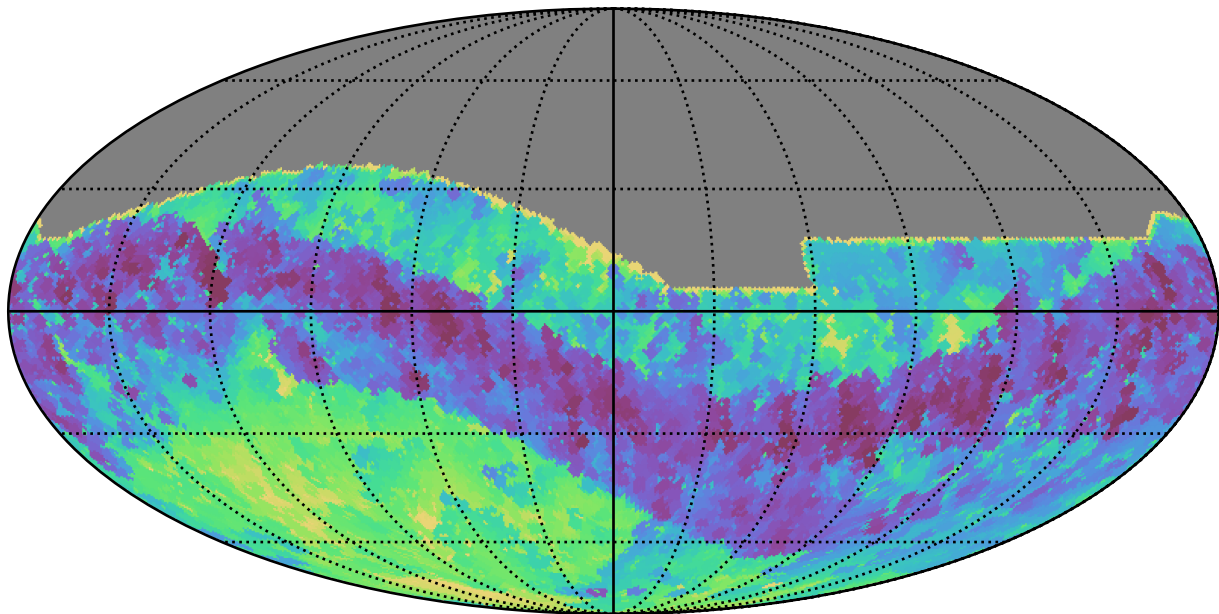
mw_roll_all_v3.3_10yrs All sky i band: Min skyBrightness
