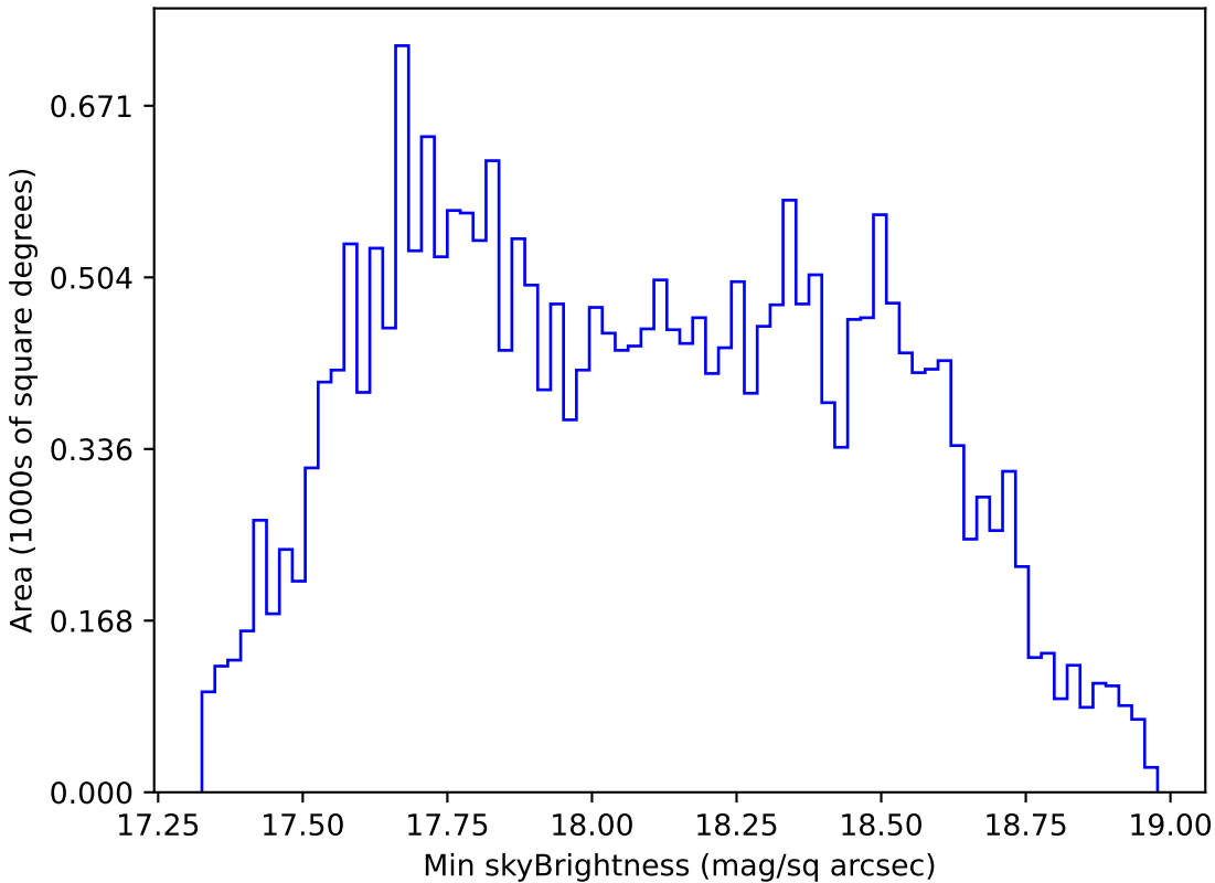
mw_roll_all_v3.3_10yrs All sky i band: Min skyBrightness
