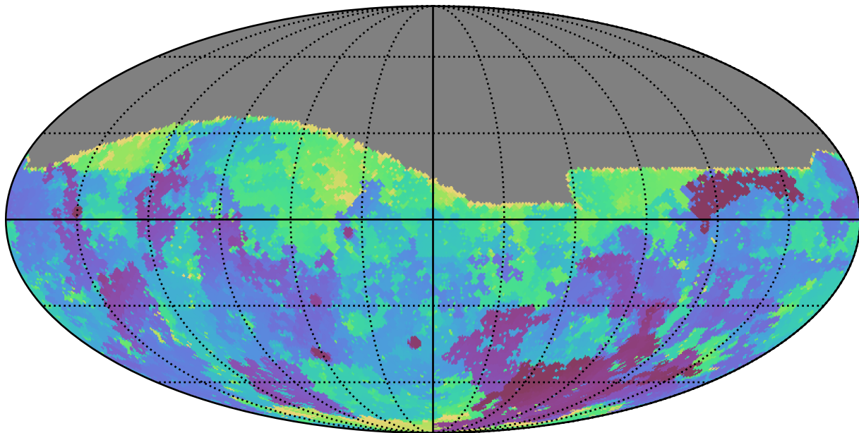
mw_roll_all_v3.3_10yrs All sky g band: Min skyBrightness
