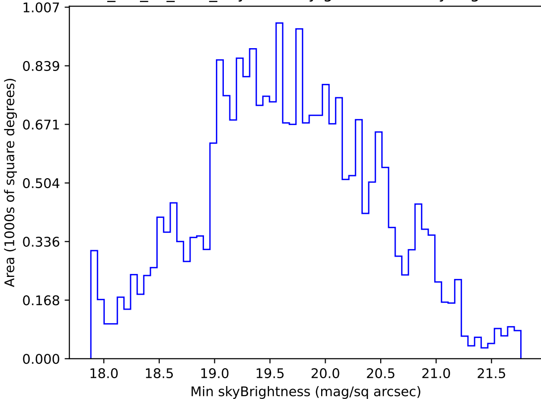
mw_roll_all_v3.3_10yrs All sky g band: Min skyBrightness
