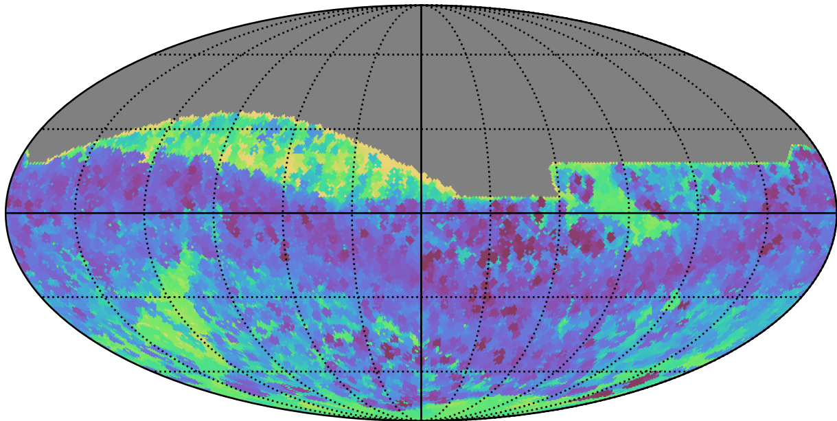
mw_roll_all_v3.3_10yrs All sky all bands: Min skyBrightness
