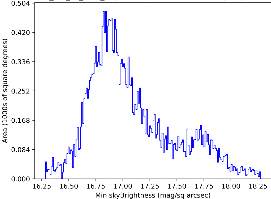
mw_roll_all_v3.3_10yrs All sky all bands: Min skyBrightness
