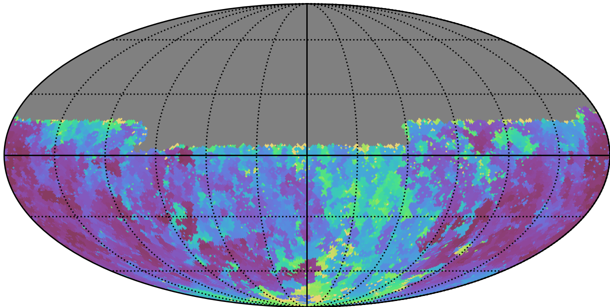
mw_roll_all_v3.3_10yrs Yr 1 u band: Min seeingGeom
