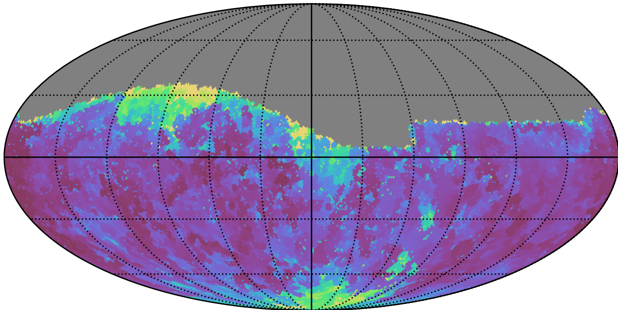
mw_roll_all_v3.3_10yrs Yr 1 g band: Min seeingGeom
