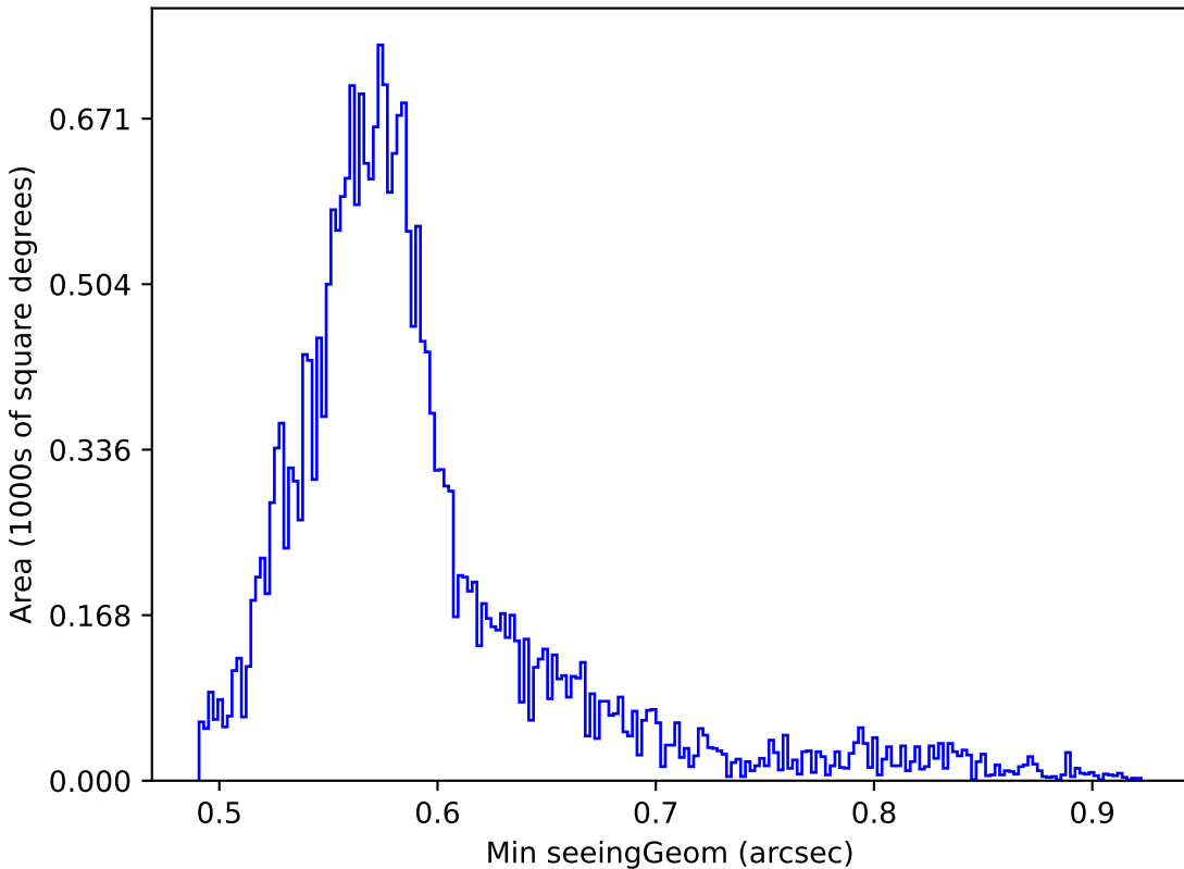
mw_roll_all_v3.3_10yrs Yr 1 all bands: Min seeingGeom
