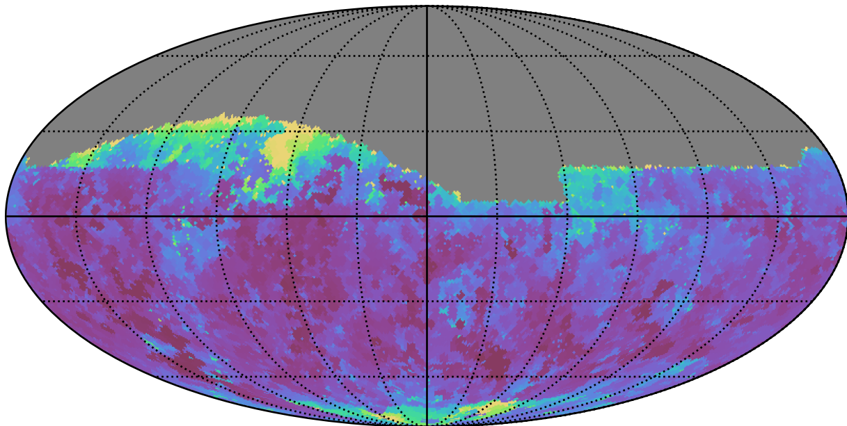
mw_roll_all_v3.3_10yrs Yr 1 z band: Min seeingEff
