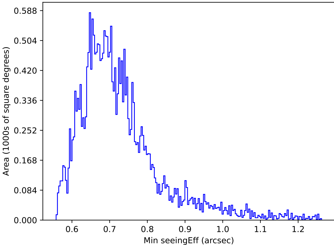
mw_roll_all_v3.3_10yrs Yr 1 z band: Min seeingEff
