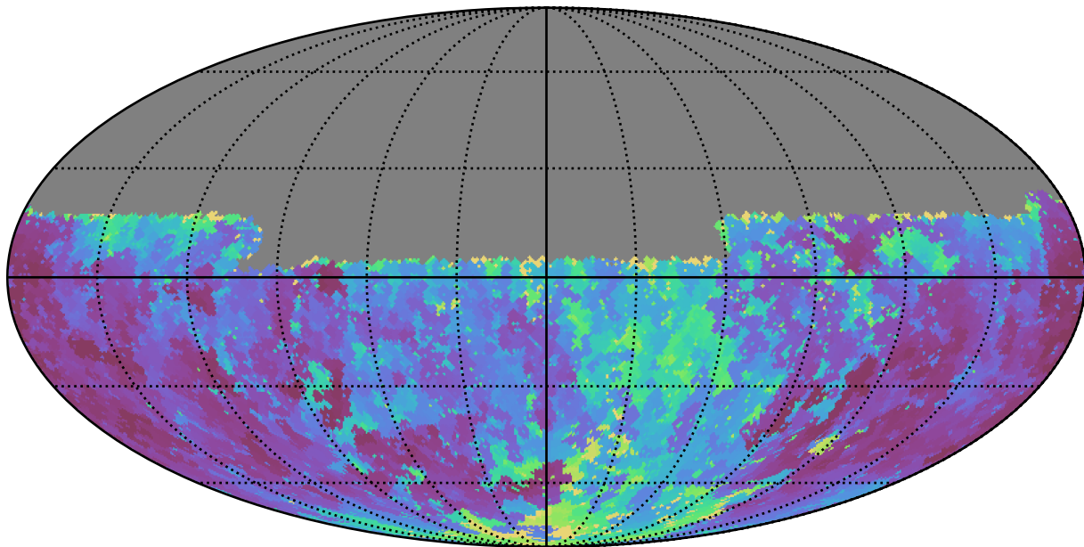
mw_roll_all_v3.3_10yrs Yr 1 u band: Min seeingEff
