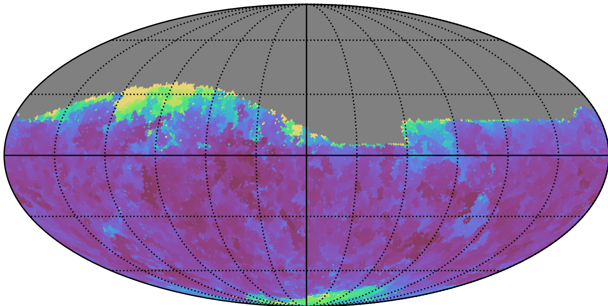
mw_roll_all_v3.3_10yrs Yr 1 r band: Min seeingEff
