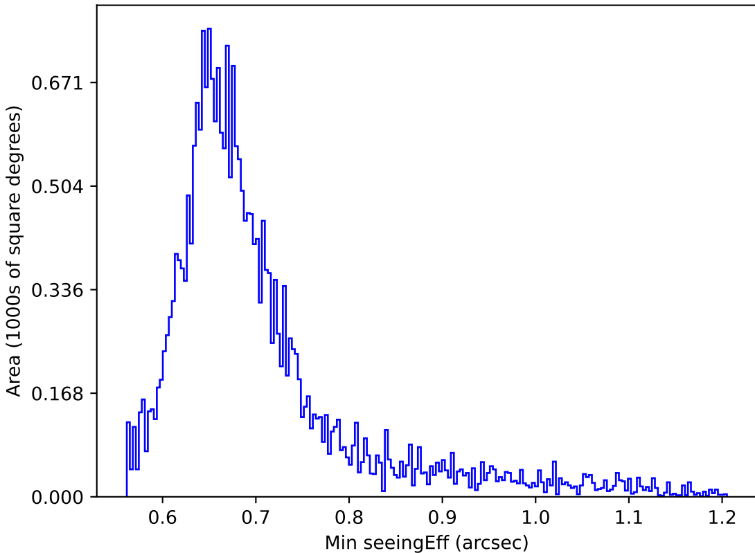
mw_roll_all_v3.3_10yrs Yr 1 i band: Min seeingEff
