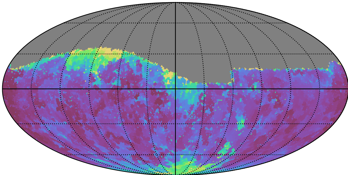
mw_roll_all_v3.3_10yrs Yr 1 g band: Min seeingEff
