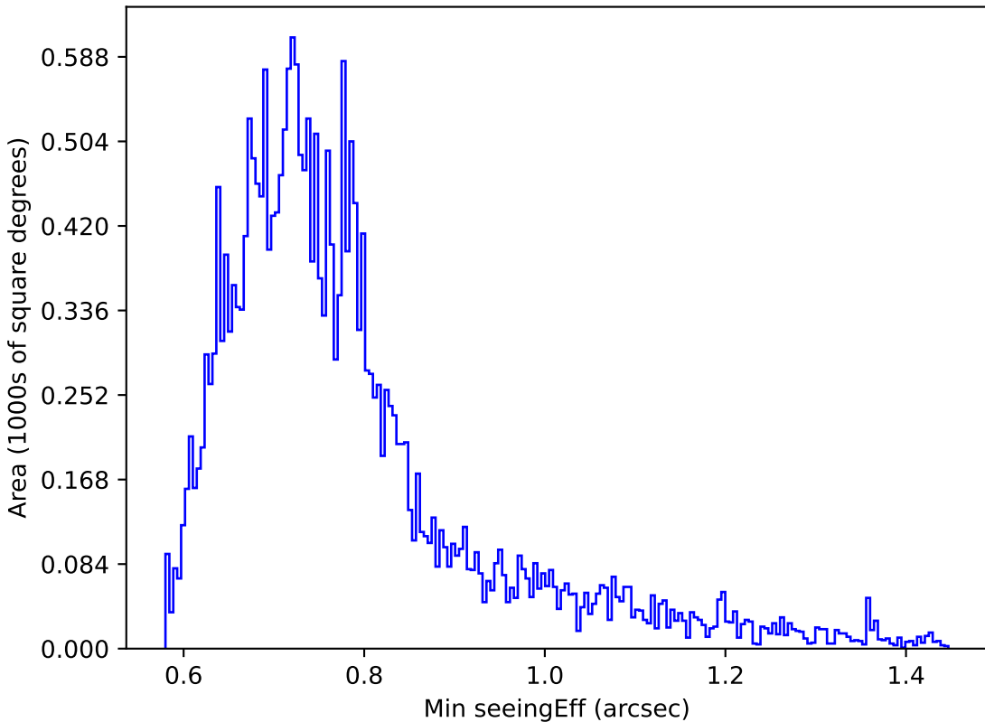
mw_roll_all_v3.3_10yrs Yr 1 g band: Min seeingEff
