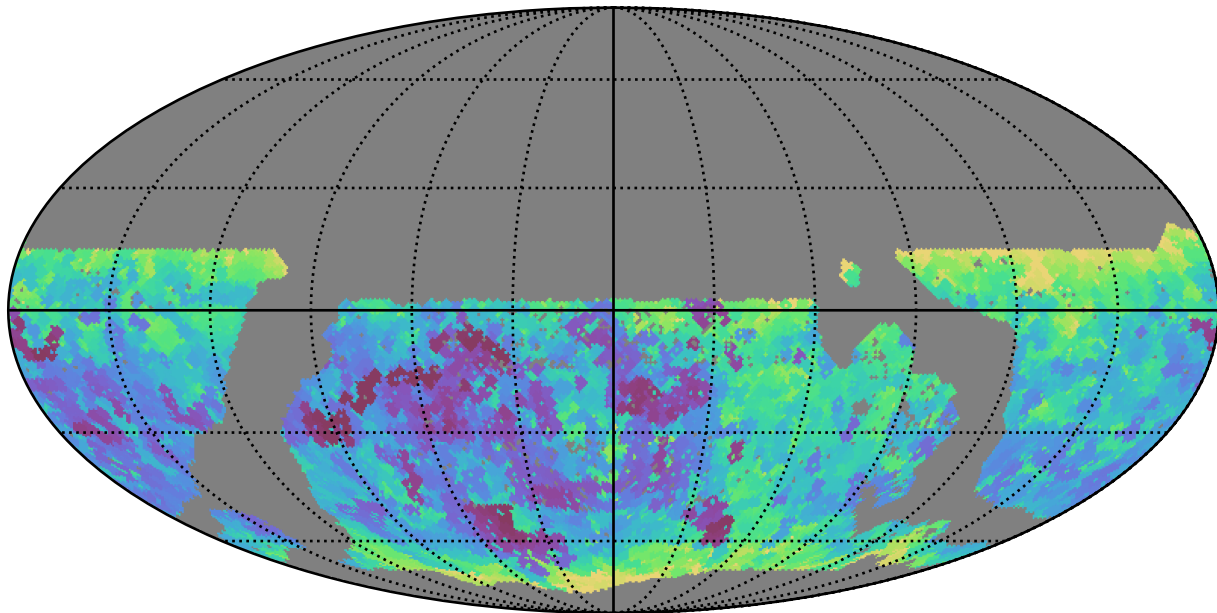
mw_roll_all_v3.3_10yrs WFD z band: Min seeingEff
