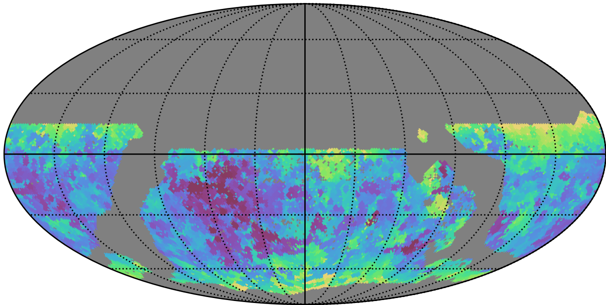
mw_roll_all_v3.3_10yrs WFD y band: Min seeingEff
