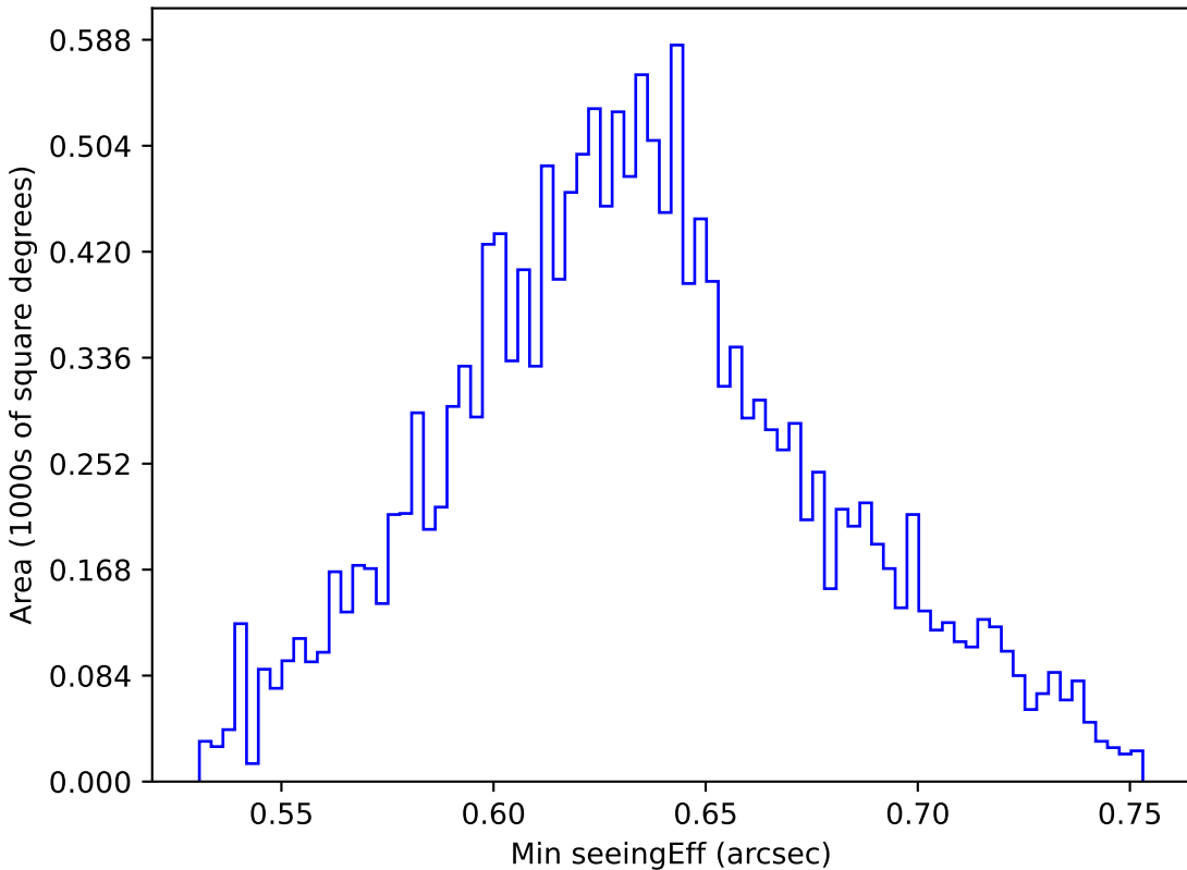
mw_roll_all_v3.3_10yrs WFD y band: Min seeingEff
