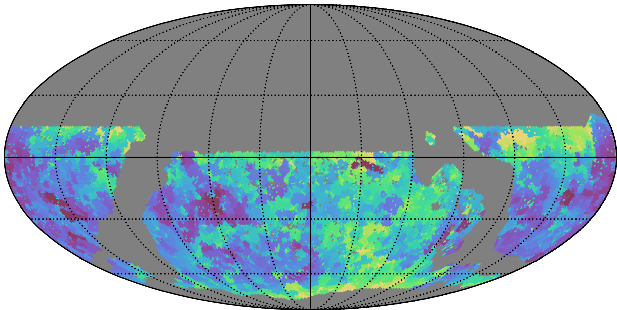
mw_roll_all_v3.3_10yrs WFD u band: Min seeingEff
