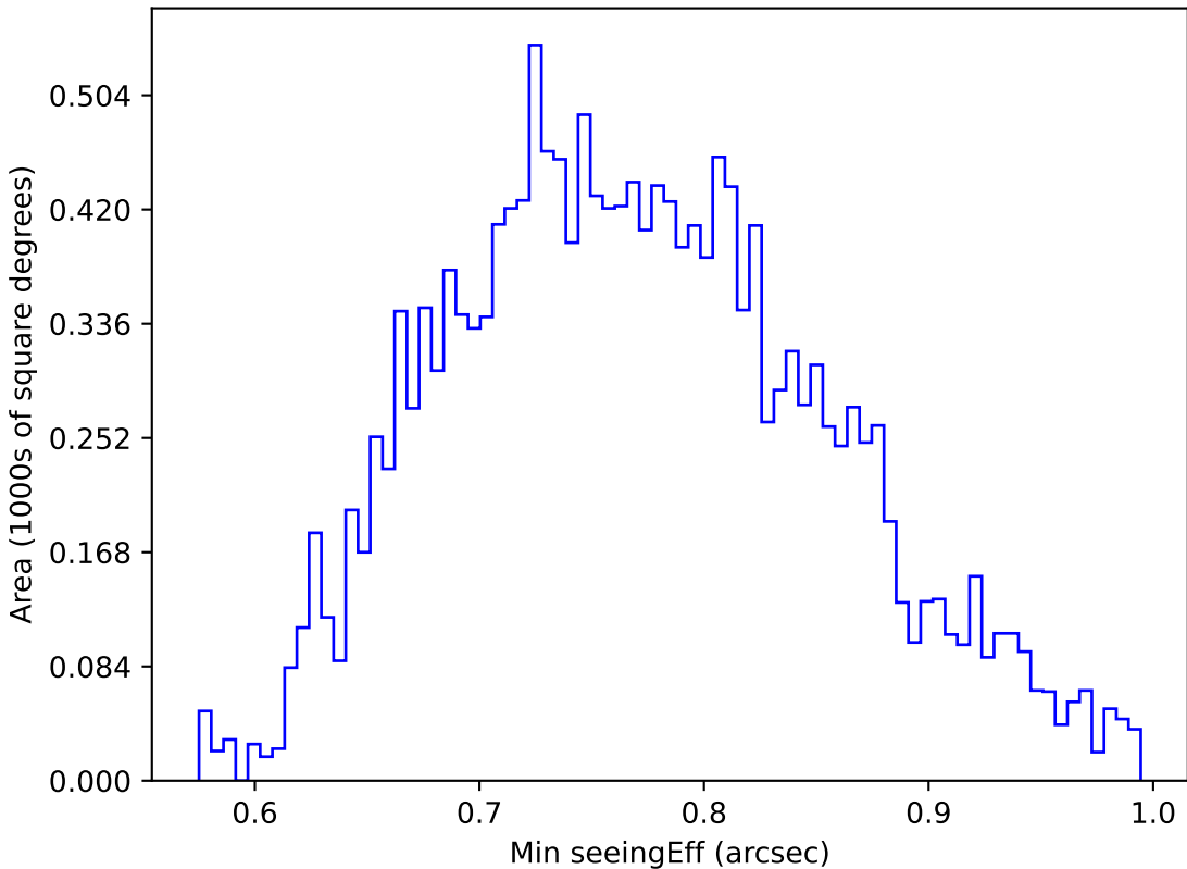
mw_roll_all_v3.3_10yrs WFD u band: Min seeingEff
