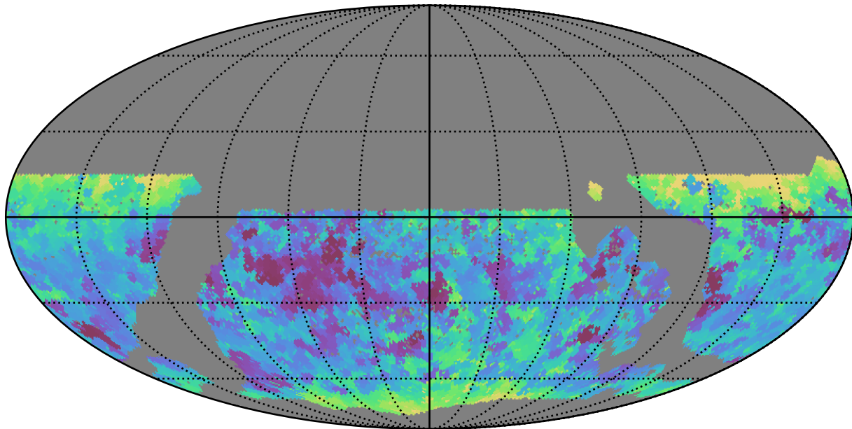
mw_roll_all_v3.3_10yrs WFD r band: Min seeingEff
