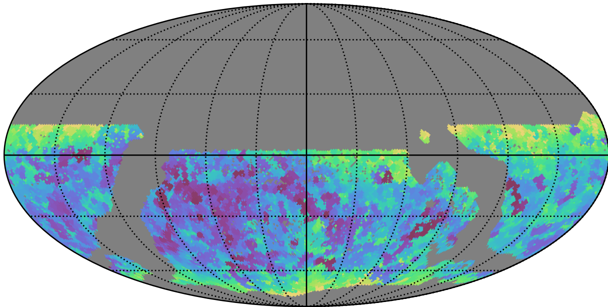
mw_roll_all_v3.3_10yrs WFD i band: Min seeingEff
