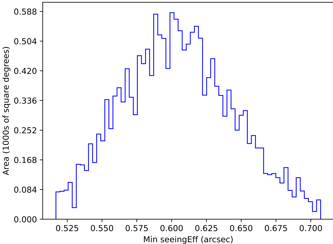
mw_roll_all_v3.3_10yrs WFD i band: Min seeingEff
