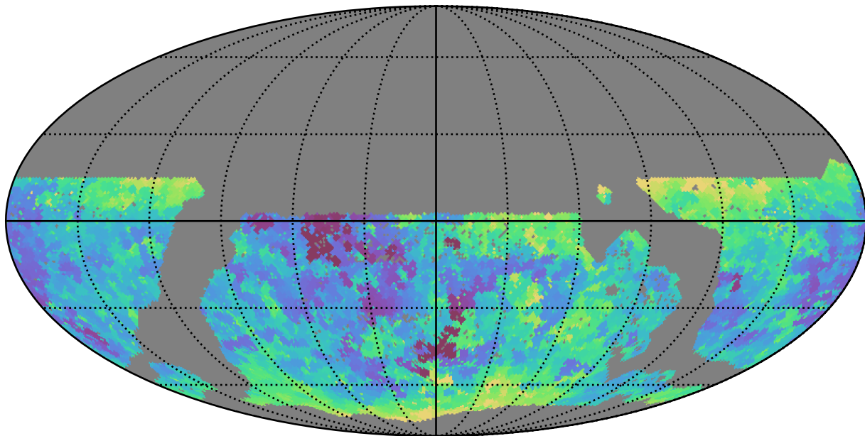
mw_roll_all_v3.3_10yrs WFD g band: Min seeingEff
